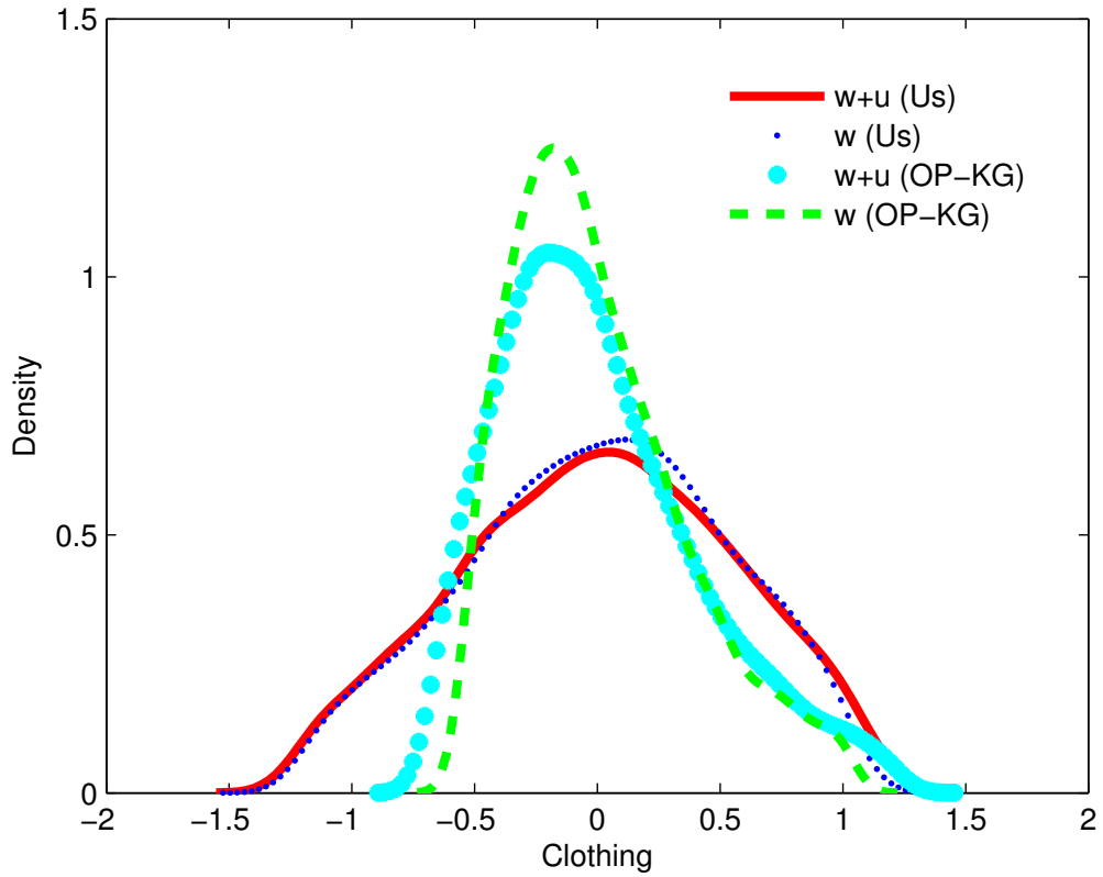
Figure A.3: Comparison: densities of \hat{\omega} and \hat{\omega} + \hat{u} – large demonstration
